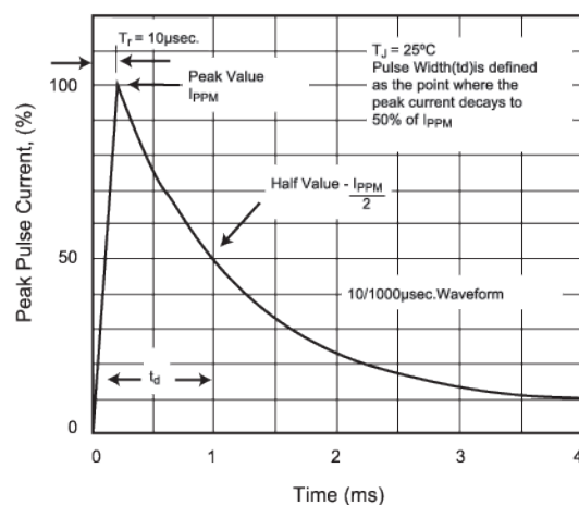
Fig. 2 - Pulse Waveform
