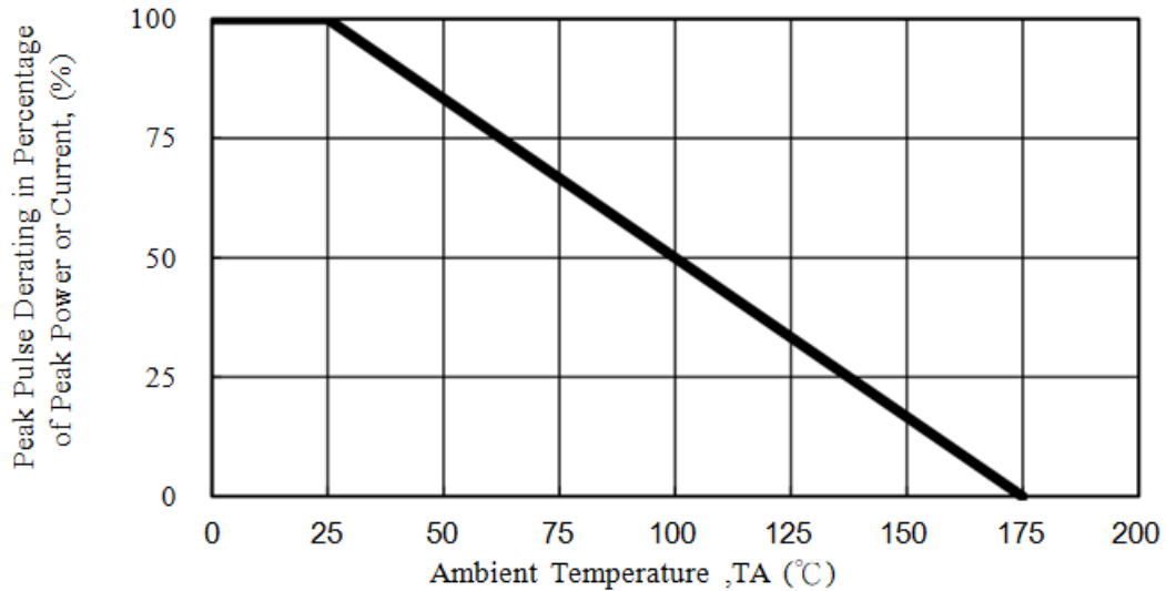
Fig. 1 - Pulse Derating Curve
