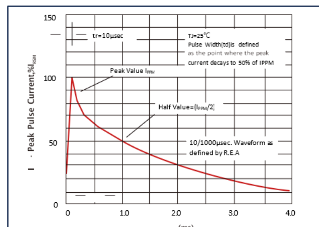
Pulse Waveform
