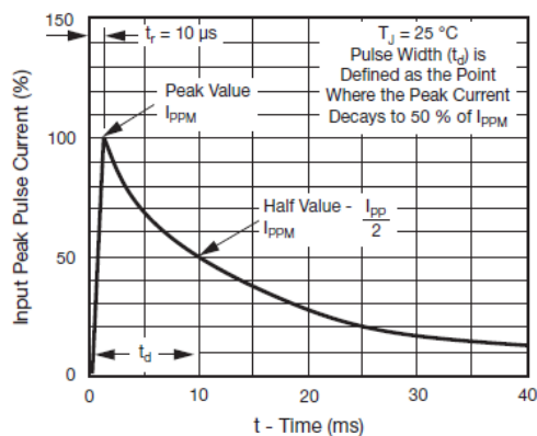
Fig. 3 - Pulse Waveform
