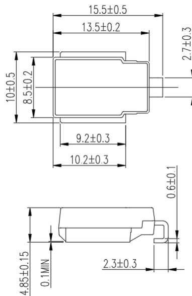
DO-218AB
