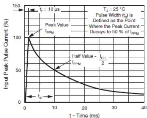
Fig. 3 - Pulse Waveform
