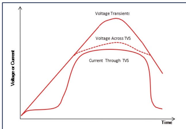
TVS Transients Clamping Waveform
