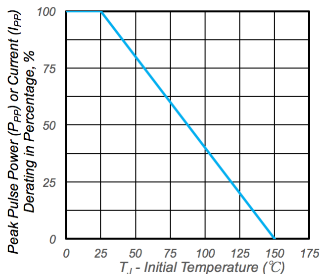
Fig.2 - Pulse Derating Cure
